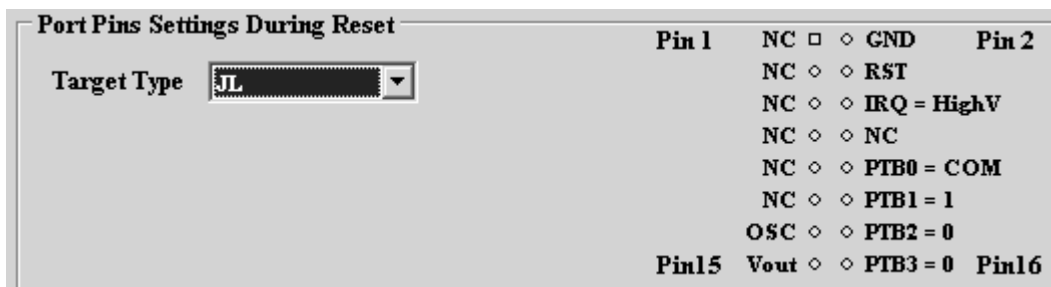
Figure 3-17: 68HC908JL Family MON08 Pinout
